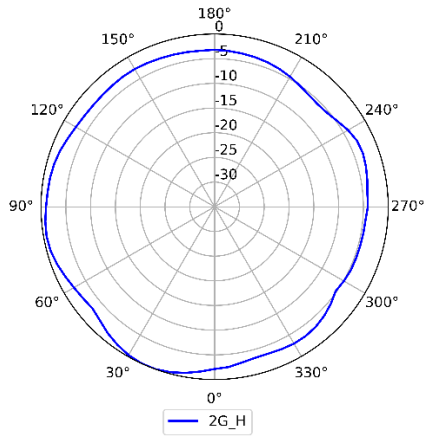
2.4GHz (Horizontal)
